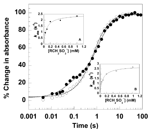
FIGURE 4: Kinetics of flavin oxidation by SsuD in the presence of octanesulfonate. Experiments were performed by stopped-flow kinetic analysis at 4 °C. Flavin oxidation of free FMNH 2 (15 \mu M) mixed with SsuD (45 \mu M) and octanesulfonate (50 \mu M) in air-saturated buffer monitored at 370 (●) and 450 nm (○). Inset A: Octanesulfonate concentration dependence on the k_{\text{obs}} for the second phase at 370 nm. Inset B: Octanesulfonate concentration dependence on the k_{\text{obs}} for the first phase at 450 nm. The kinetic traces shown are the average of three separate experiments. The solid lines are the fits of the kinetic traces to eq 3 or 4.
